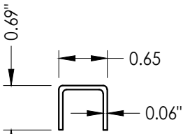
53 GLASS STOP
