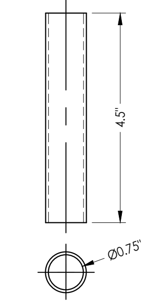
83 SILL TUBE ANCHOR
