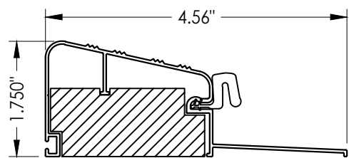
78 OUTSWING THRESHOLD
